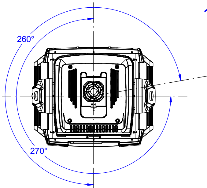
Pan movement range:530°
