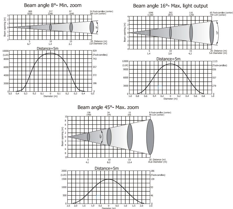
Lamp: Halogen lamp 750W/80V
