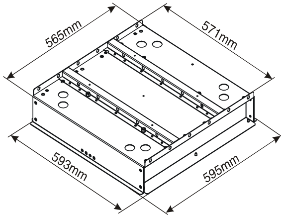
Ceiling box 99010551
