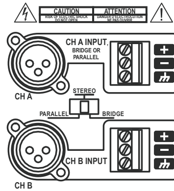
XLR and Terminal Block inputs
