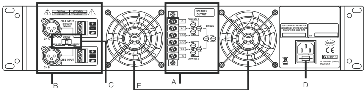
XLR and Terminal Block inputs
