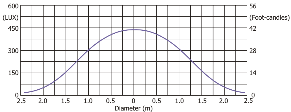
Beam angle 40° with frost, distance=5m
